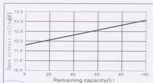
Curves of open circuit voltage vs. capacity
