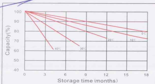
Curves of self discharge
